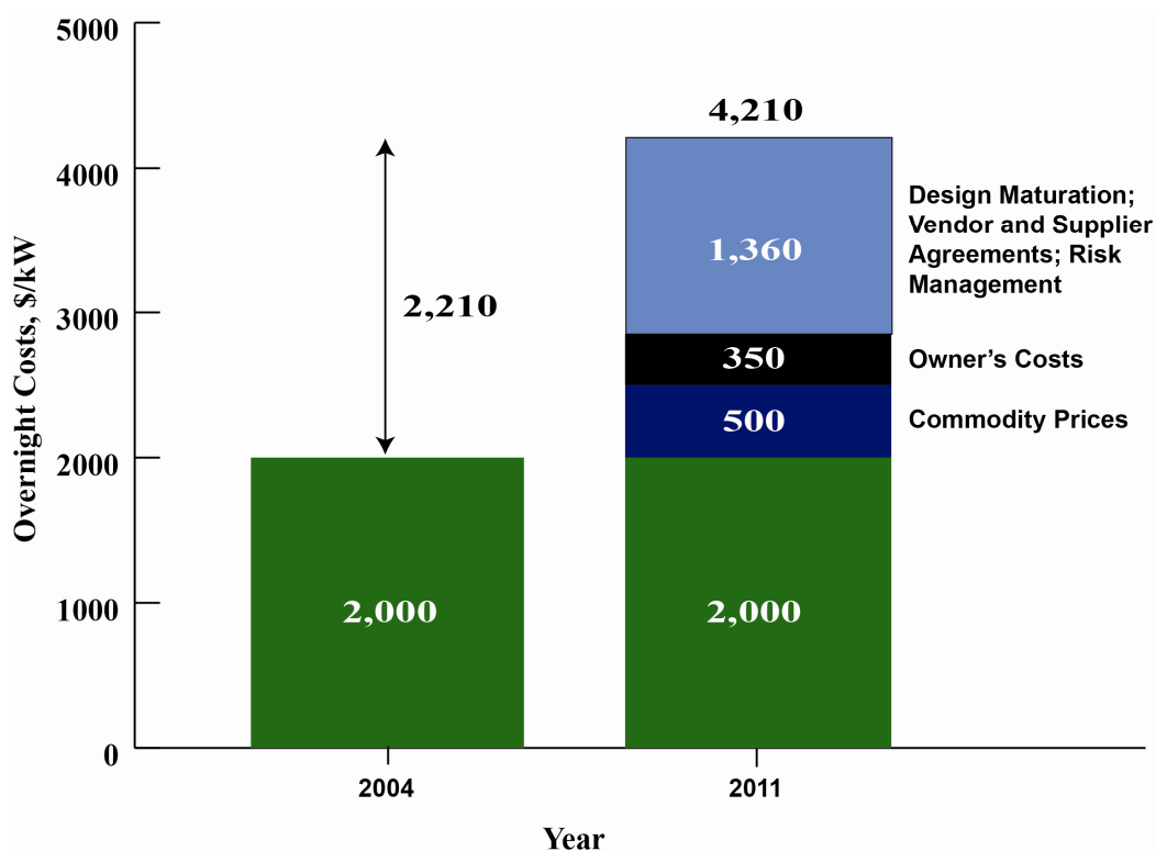
FIGURE 1 Overnight Cost Change (2011$) for GW-LWRs
