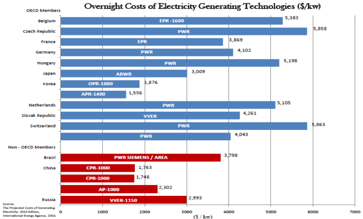
Figure D-1 Overnight Costs of Electricity Generating Technologies ($/kW). (Reproduced with permission.)
