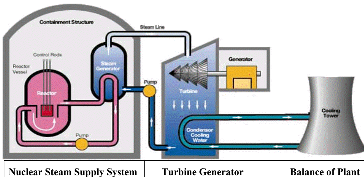
FIGURE 2 Schematic Diagram of a Pressurized Water Reactor
