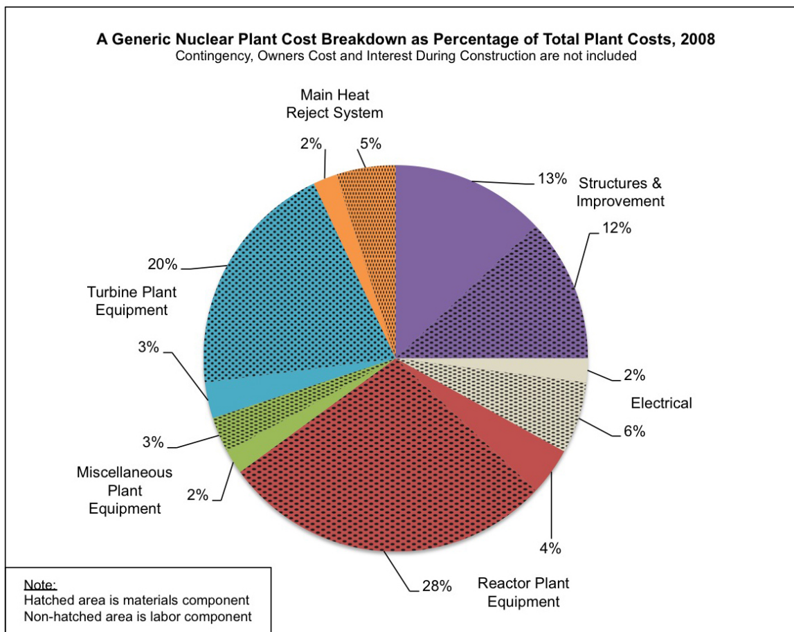
FIGURE E-1 Breakdown of Nuclear Power Plant Costs by Major Components (from EPRI). (Reproduced with permission.)
